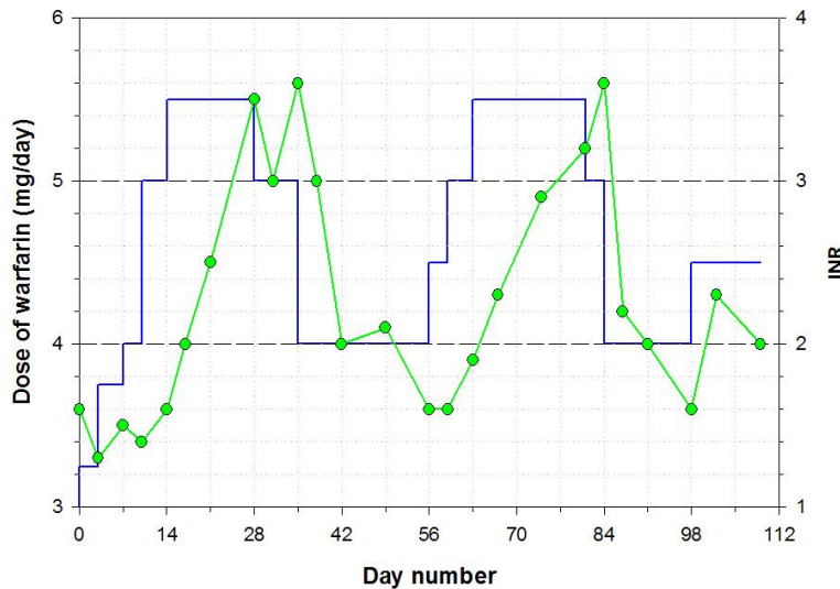
Figure 2. History of dosage (blue line) and INR (green line) over three and a half months for Patient #23. The dose was changed whenever the INR was outside the therapeutic range of 2.0 to 3.0; this occurred on 52% of the measurements. The INR is estimated to lag the dose by about 15 days.
