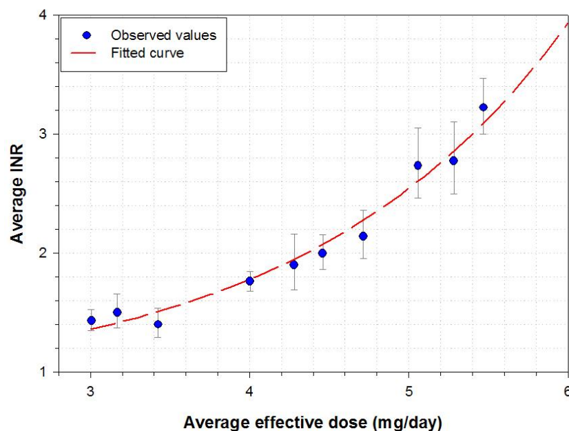
Figure 3. Dose-effect curve for Patient #23. The effective dose is a weighted average of previous doses. Effective doses were combined into groups according to the nearest multiple of 0.25 mg; the observed values are the means for each group.
