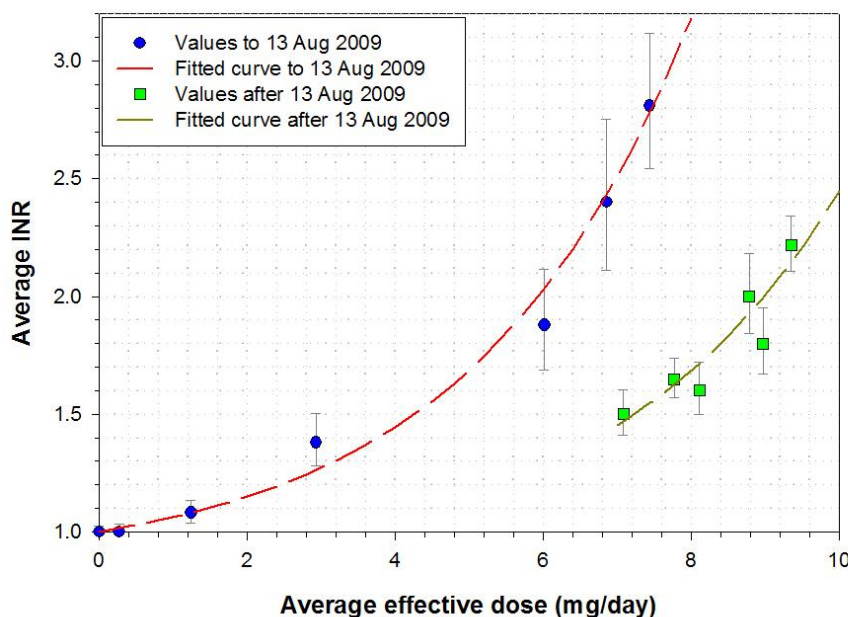
Figure 5. Dose-effect curves for Patient #1. The therapeutic range is 2.0 to 3.0. After 13 August 2009 the INR seems to have been affected by interaction with niacin and/or spironolactone.
