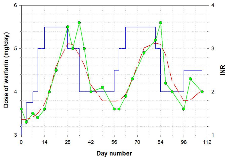
Figure 4. History of dosage (blue line) and INR (green line) over three and a half months for Patient #23, and the average INR predicted (red line) from the dose-effect curve shown in Figure 3.
